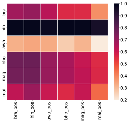
(a) Lexical similarity of monolingual corpus with POS dataset (mono-POS overlap)
