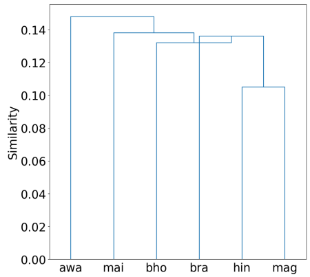
(b) Dendrogram from pairwise transfer results with fixed dataset sizes
